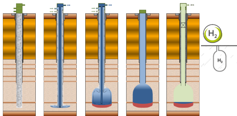
Solution mining of a salt cavern for H 2 storage
